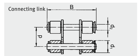
Design LR double pitch
