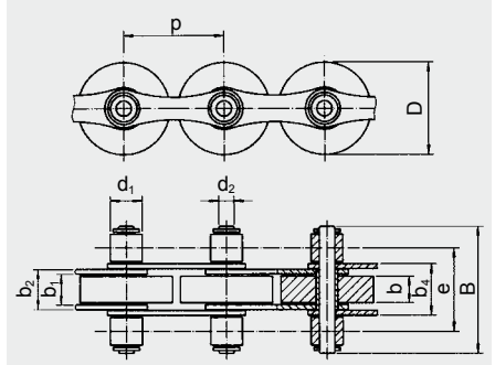
Design LR double pitch
