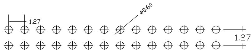
PCB LAYOUT
