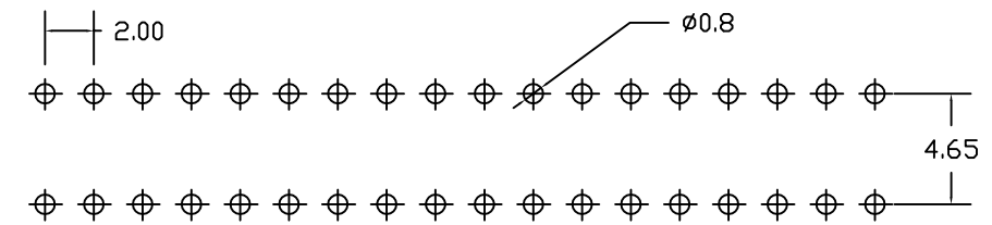
PCB LAYOUT
