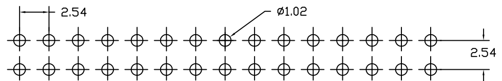
PCB LAYOUT
