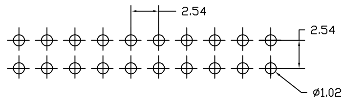
PCB LAYOUT
