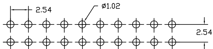
PCB LAYOUT
