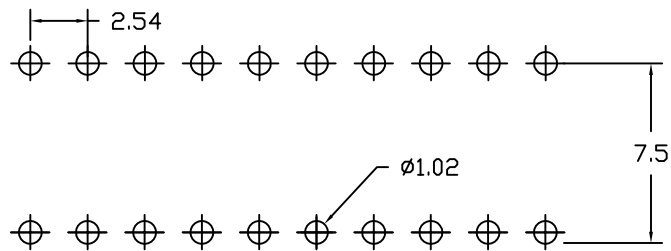
PCB LAYOUT
