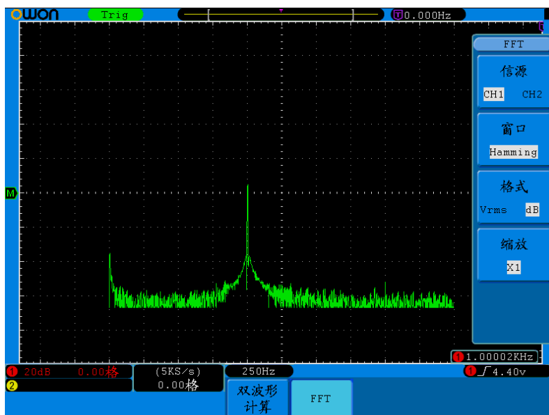
图5-11. HAMMING窗
