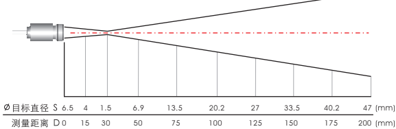
CSmicro 3ML CF1, D:S=22:1 (远距离3.5:1)
