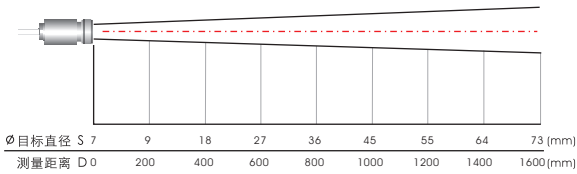
CSmicro 3ML CF, D:S=22:1 (远距离9:1)
