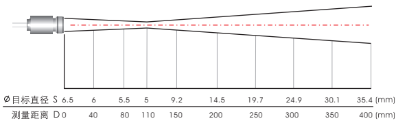
CSmicro 3ML CF1, D:S=22:1 (远距离3.5:1)
