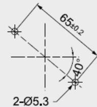
Mounting Dimensions
