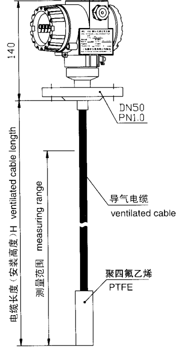
法兰安装 耐酸碱型 flange connecting, acid and alkali resistant type
