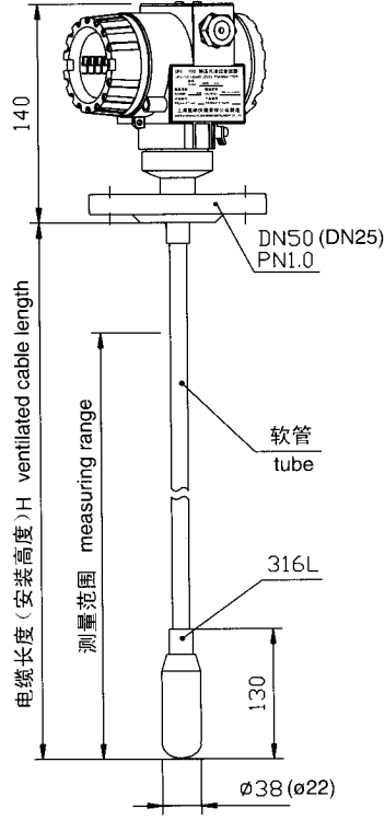
法兰安装 耐油型 flange connecting, oil resistant type
