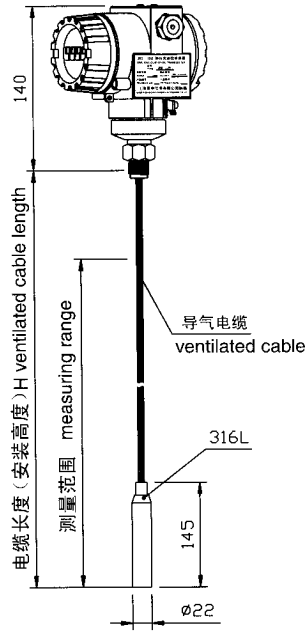
螺纹安装 细径型 thread connecting, slender type
