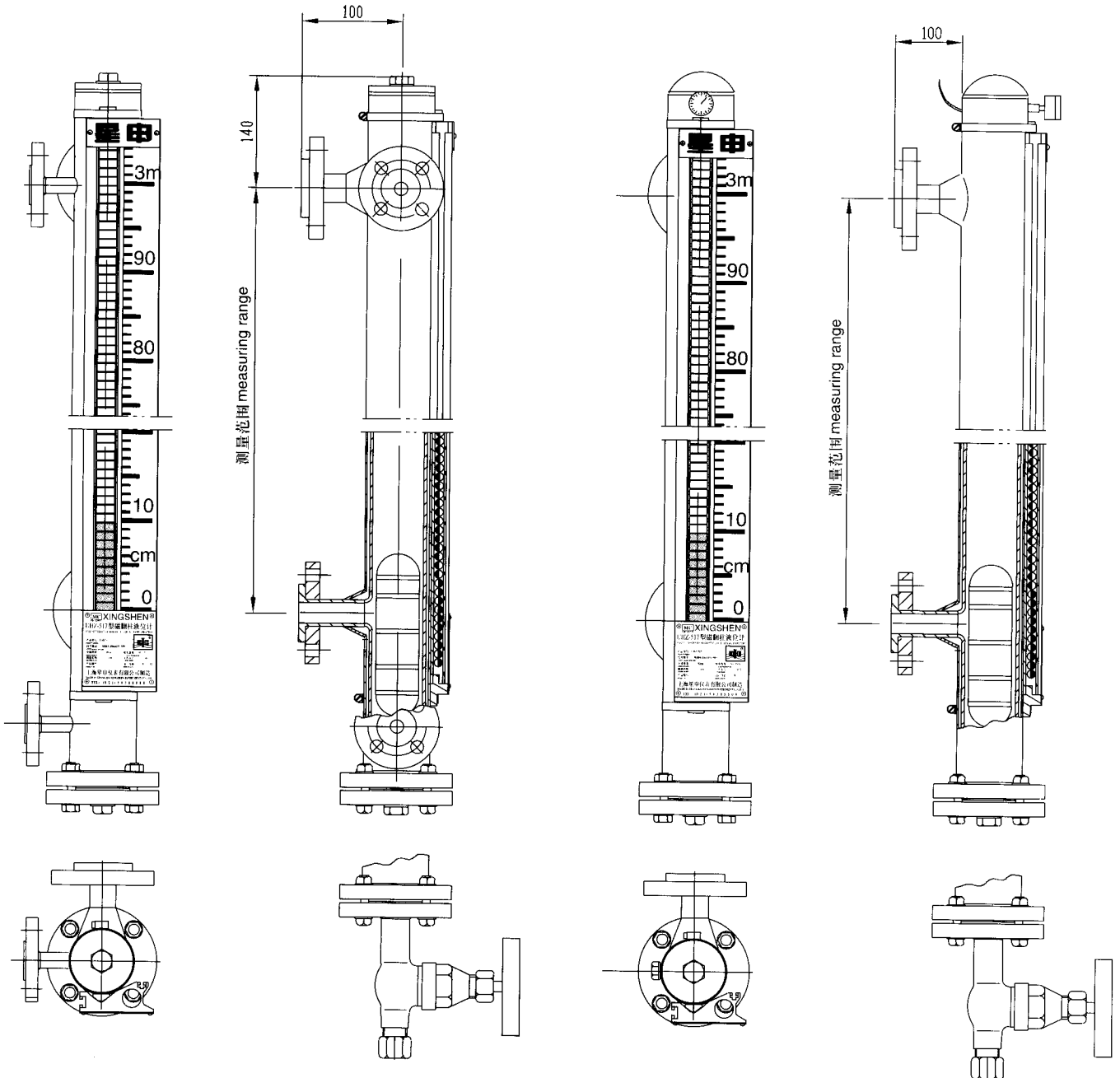
蒸汽夹套，水循环夹套 steam jacket and cycling water jacket
