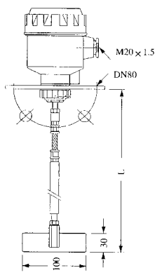
UZK-A32(轴长可调型) axis length adjustable type
