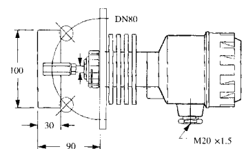
UZK-A12H(高温型) high temperature type
