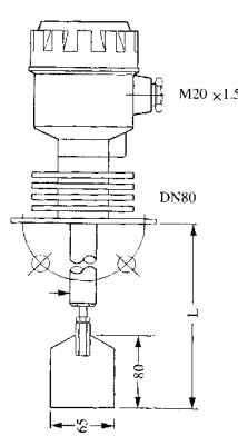
UZK-B22H(轴保护管高温型) axis protection tube, high temperature type
