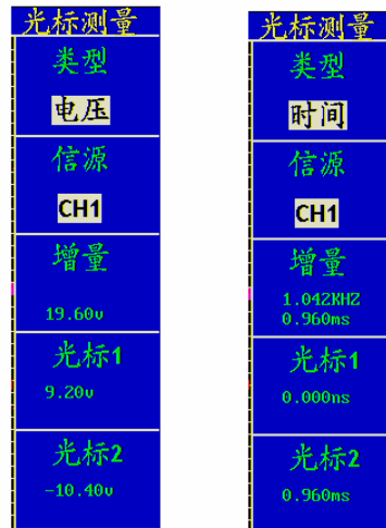
图5-45: 光标测量菜单
