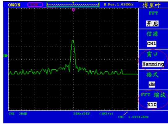
图5-12. HAMMING窗
