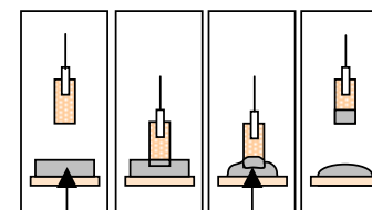
Solder Paste Heating
