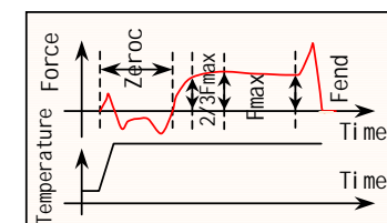
Mol ten solder Rapid heating
