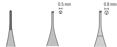
Serrated Tip width: 0.8 mm No. 11020-12 1x2 teeth Tip width: 0.5 mm No. 11032-12 1x2 teeth with platform Tip width: 0.8 mm No. 11022-12
