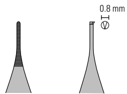
Serrated No. 11018-12 1x2 teeth No. 11019-12
