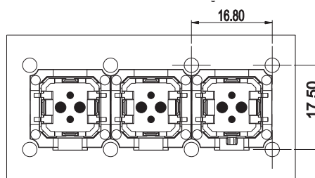
Kleinster Raster / Minimum grid: 16.80 x 17.50
