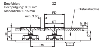
SMT gullwing terminal
