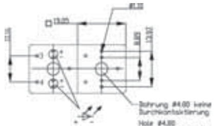
Momentary key switch, non-illuminated
