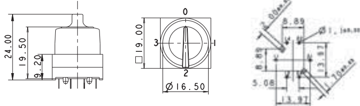
PCB hole pattern, component side
