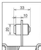
● SA-4602 附带阻挡橡胶
