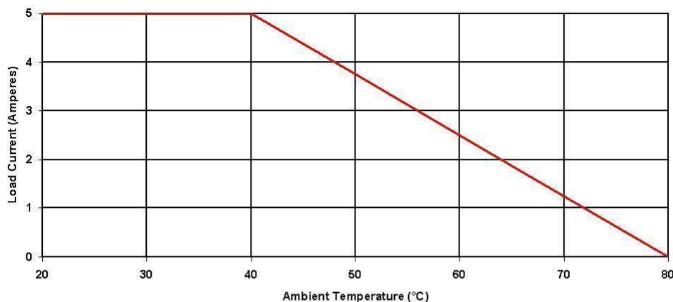
DERATING CURVE: EDxx5
