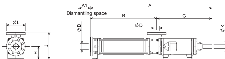
Diagram 4. Models AF, Build H and AG Build M. Cast Iron and Stainless Steel.
