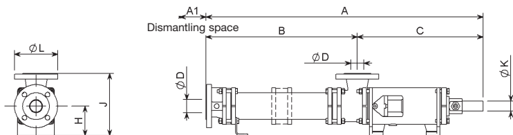
Diagram 1. Models AA, AB, AC & AE. Typical Builds H and M. Cast Iron and Stainless Steel
