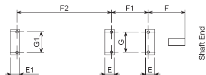
Foundation Fixing Details
