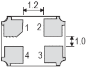
Underside View
