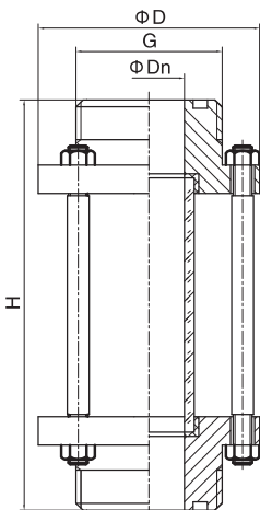
视镜 Sight glass
