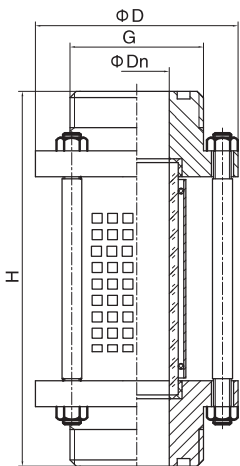
防护网视镜 Sight glass with protective net
