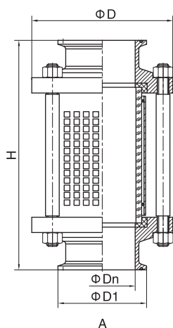
防护网视镜 Sight glass with protective net
