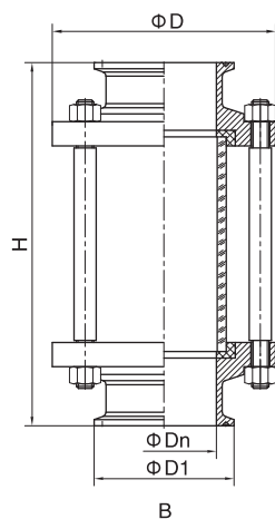
视镜 Sight glass
