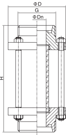
视镜 Sight glass
