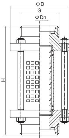
防护网视镜 Sight glass with protective net
