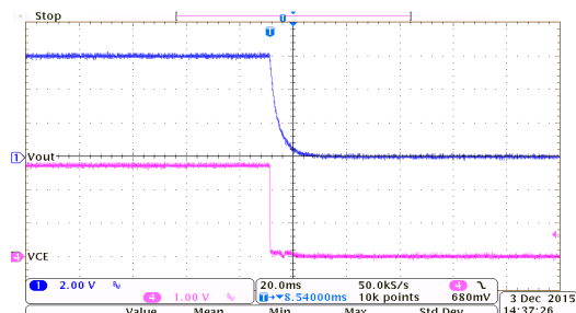
ON/OFF Response: HT7560-7 ( I_{OUT}=0mA , V_{CE}=2.7V to 0V)
