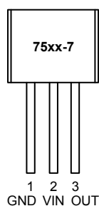
TO92-3
