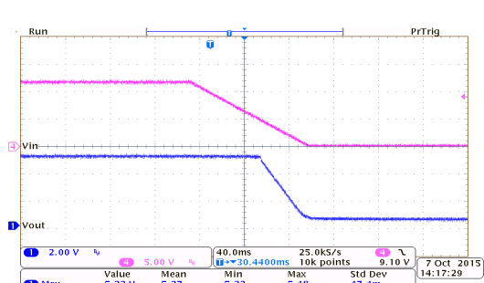
Power Off Response: HT7550-7 ( I_{OUT}=150mA , T_{FALL}=100ms )
