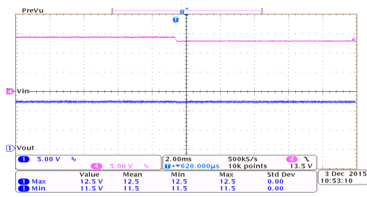
Line Transient Response: HT75C0-7 ( I_{OUT}=10mA )
