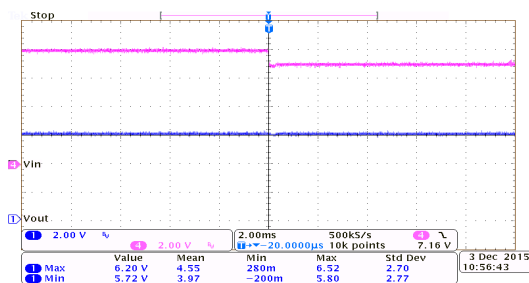
Line Transient Response: HT7560-7 ( I_{OUT}=10mA )
