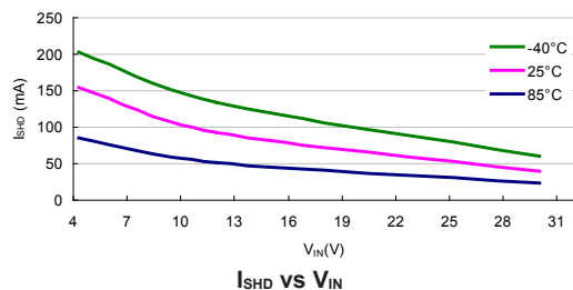
I_{SHD} vs V_{IN}
