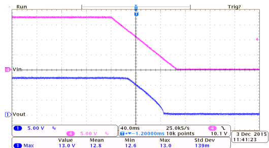
Power Off Response: HT75C0-7 ( I_{OUT}=150mA , T_{FALL}=100ms )
