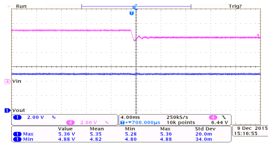
Line Transient Response: HT7550-7 ( I_{OUT}=10mA )
