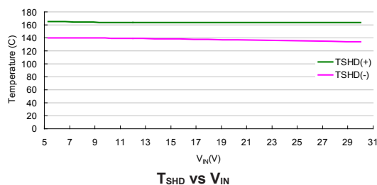
T_{SHD} vs V_{IN}
