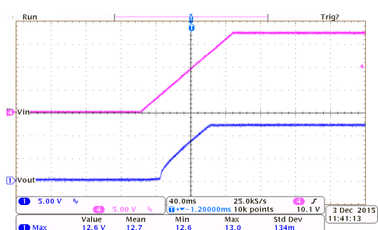
Power On Response: HT75C0-7 ( I_{OUT}=150mA , T_{RISE}=100ms )
