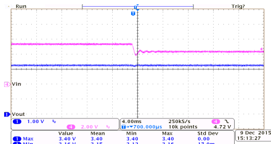
Line Transient Response: HT7533-7 ( I_{OUT}=10mA )
