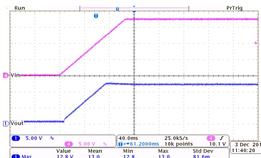
Power On Response: HT75C0-7 ( I_{OUT}=0mA , T_{RISE}=100ms )
