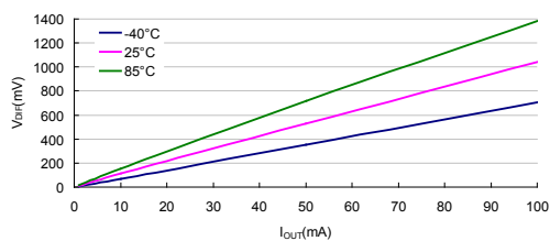
Dropout voltage: HT7533-7
