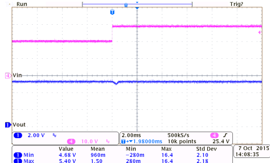
Line Transient Response: HT7550-7 ( I_{OUT}=10mA )
