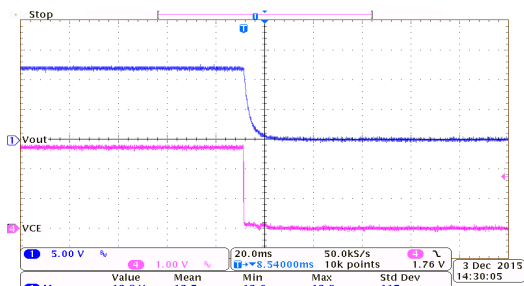
ON/OFF Response: HT75C0-7 ( I_{OUT}=0mA , V_{CE}=2.7V to 0V)
