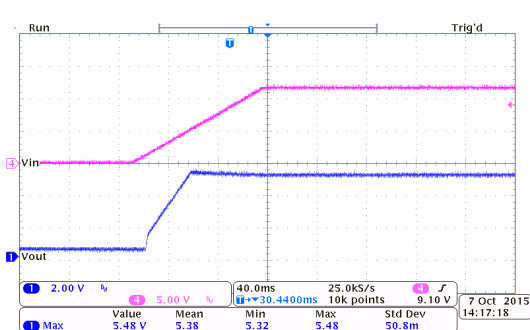
Power On Response: HT7550-7 ( I_{OUT}=150mA , T_{RISE}=100ms )
