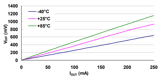
Dropout Voltage: HT7333-2
