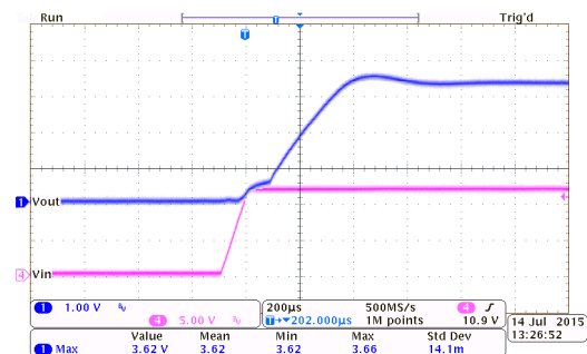
Power On Response: HT7333-2 ( I_{OUT}=250mA , T_{RISE}=0.1ms )
