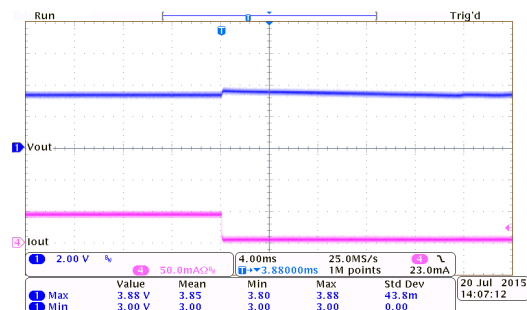
Load Transient Response: HT7333-2 ( V_{IN}=5.3V , I_{OUT}=40mA to 0mA )
