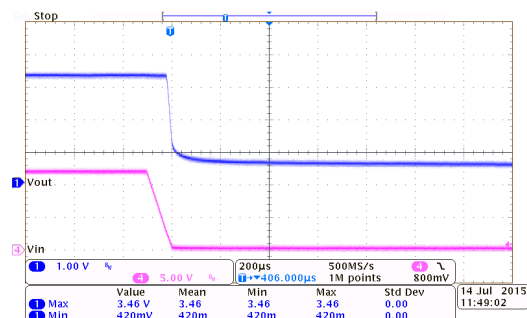
Power Off Response: HT7333-2 ( I_{OUT}=0mA , T_{FALL}=0.1ms )
