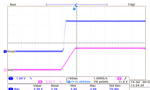
Power On Response: HT7333-2 ( I_{OUT}=250mA , T_{RISE}=100ms )
