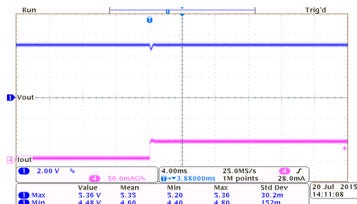
Load Transient Response: HT7350-2 ( V_{IN}=7.0V , I_{OUT}=0mA to 40mA )
