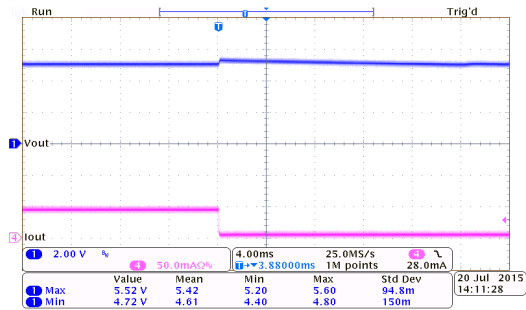
Load Transient Response: HT7350-1 ( V_{IN}=7.0V , I_{OUT}=40mA to 0mA )
