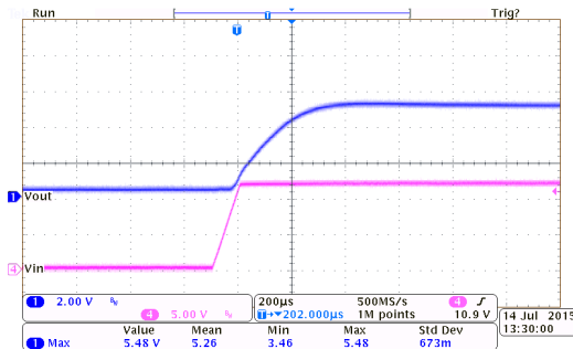
Power On Response: HT7350-1 ( I_{OUT}=0mA , T_{RISE}=0.1ms )
