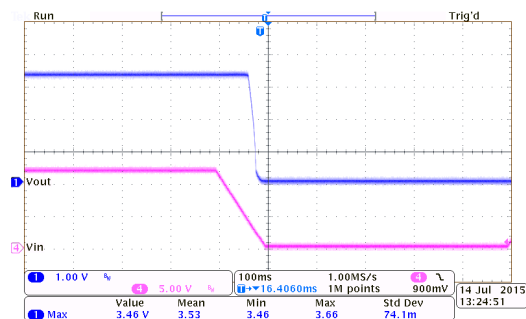
Power Off Response: HT7333-1 ( I_{OUT}=250mA , T_{FALL}=100ms )
