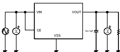
Circuit ④
