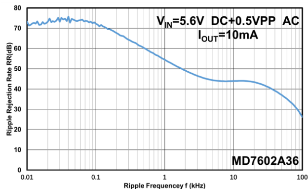
Power Supply Rejection Ratio at V_{OUT}=3.6V
