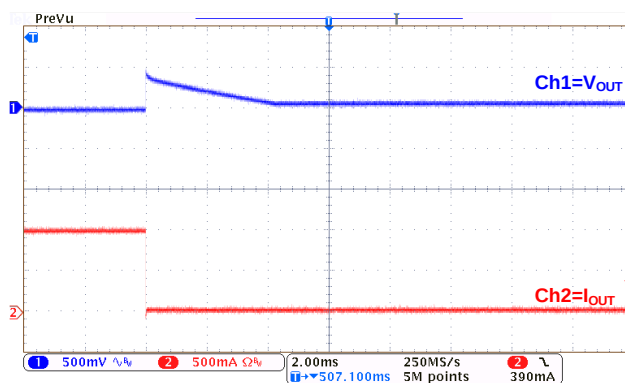
Load Transient at V_{OUT}=3.6V 7602A36( I_{OUT}=1A\sim 0mA )
