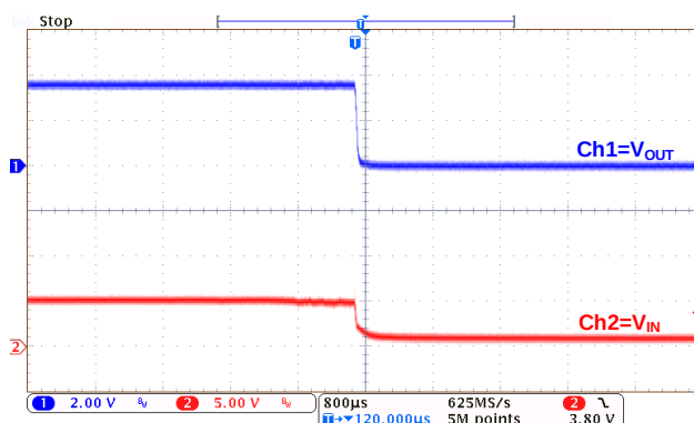
Power- Down at V_{OUT}=3.6V 7602A36( I_{OUT}=1A )
