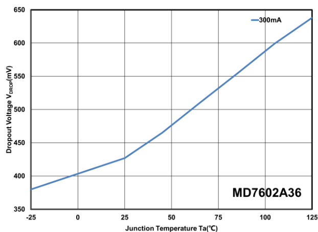
V_{DROP} vs Temperature at V_{OUT}=3.6V
