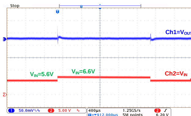
Line Transient at V_{OUT}=3.6V 7602A36( I_{OUT}=10mA )
