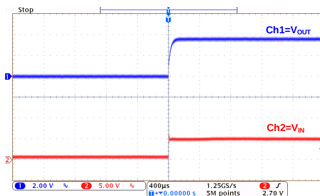
Power-Up at V_{OUT}=3.6V 7602A36( I_{OUT}=1A )
