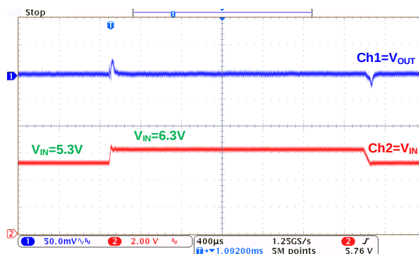
Line Transient: MD8433( I_{OUT}=1mA )
