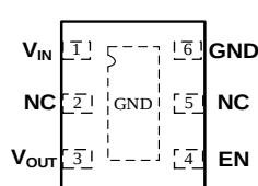
DFN(2*2)-6 Top View
