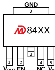
TO252-4 Top View
