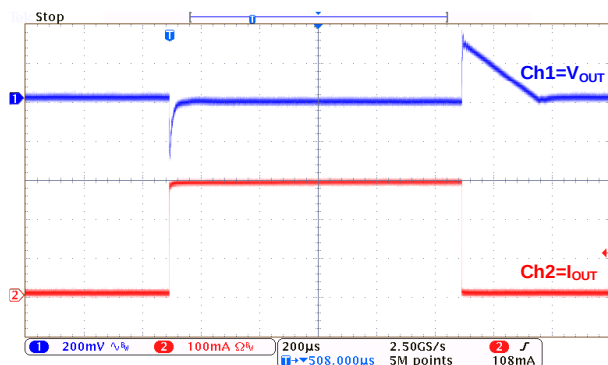
Load Transient: MD8433( I_{OUT}=1mA\sim 300mA\sim 1mA )
