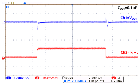
Load Transient: MD5130 ( I_{OUT}=1mA\sim 10mA\sim 1mA )
