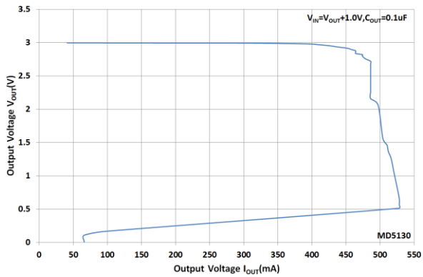
MD5130 Output Current Fold-back
