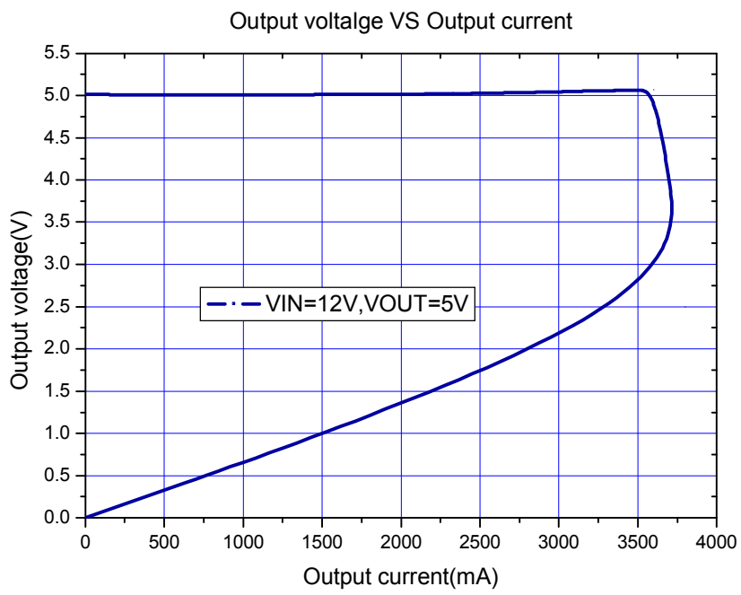
Figure6. XL2013 System Output Constant Current Curve
