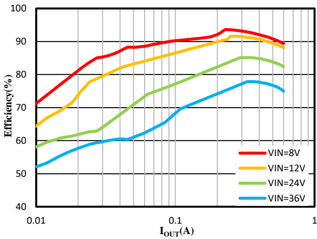
Figure 1. Efficiency, V_{OUT}=5V
