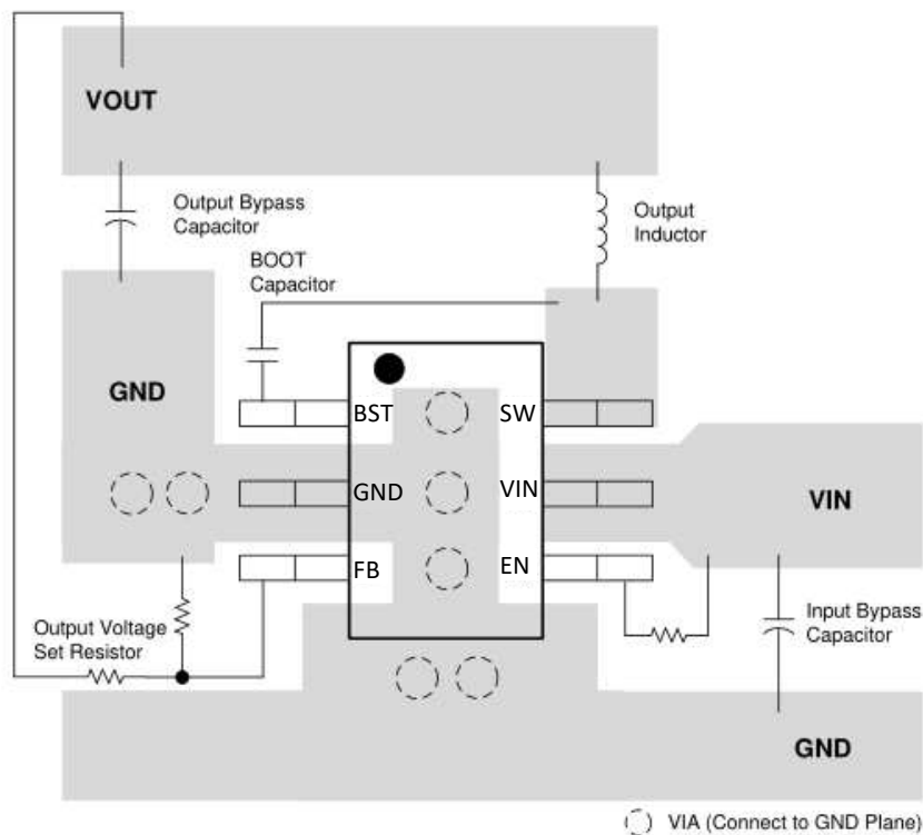
Figure 22 Layout Example
