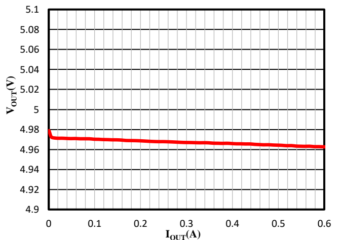
Figure 4. Load Regulation
