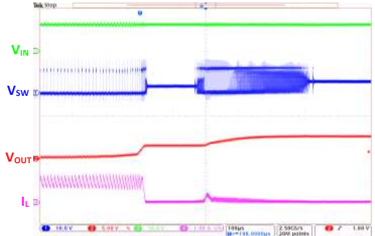
Figure 20. Short Circuit Recovery, I_{OUT} = \text{Short} to 0A
