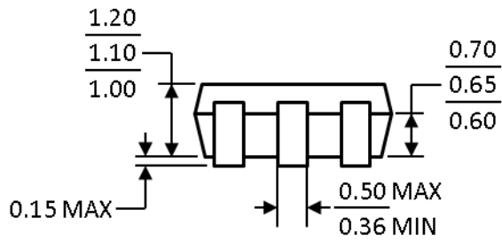
Figure 23 6-Lead Small Outline Transistor Package [SOT-23]
