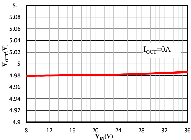
Figure 3. Line Regulation
