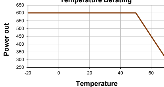
Temperature Derating
