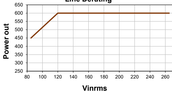
Line Derating
