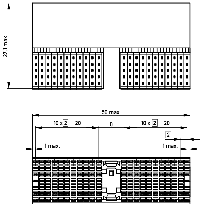
CONTACT LAYOUT
