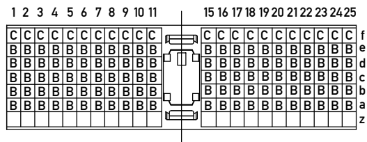
CONTACT LAYOUT
