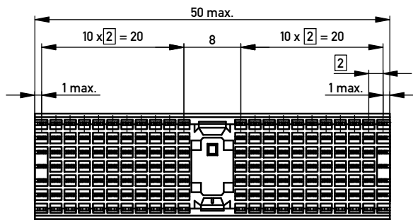
CONTACT LAYOUT
