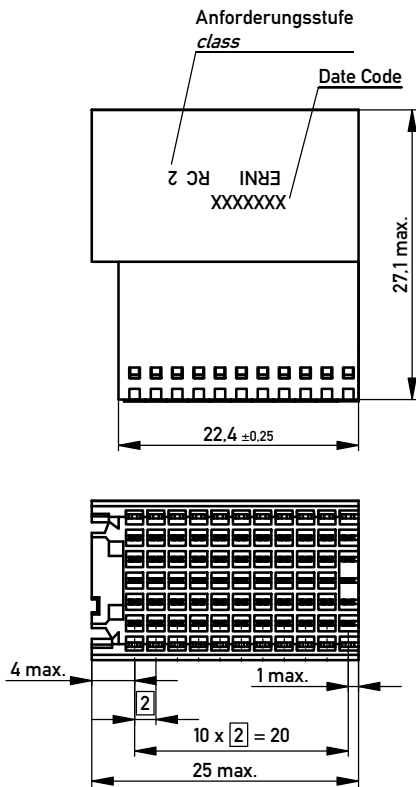
CONTACT LAYOUT
