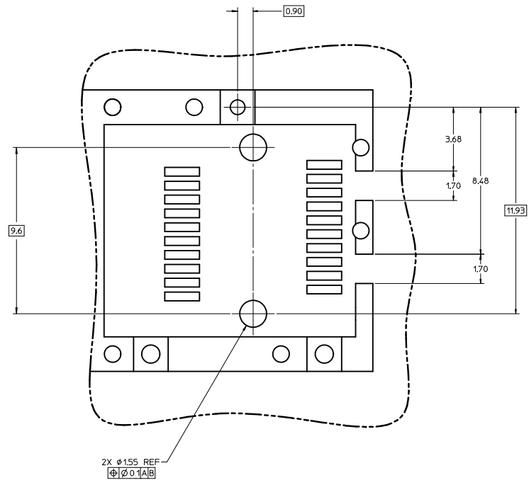
DETAIL1 SCALE 10:1
