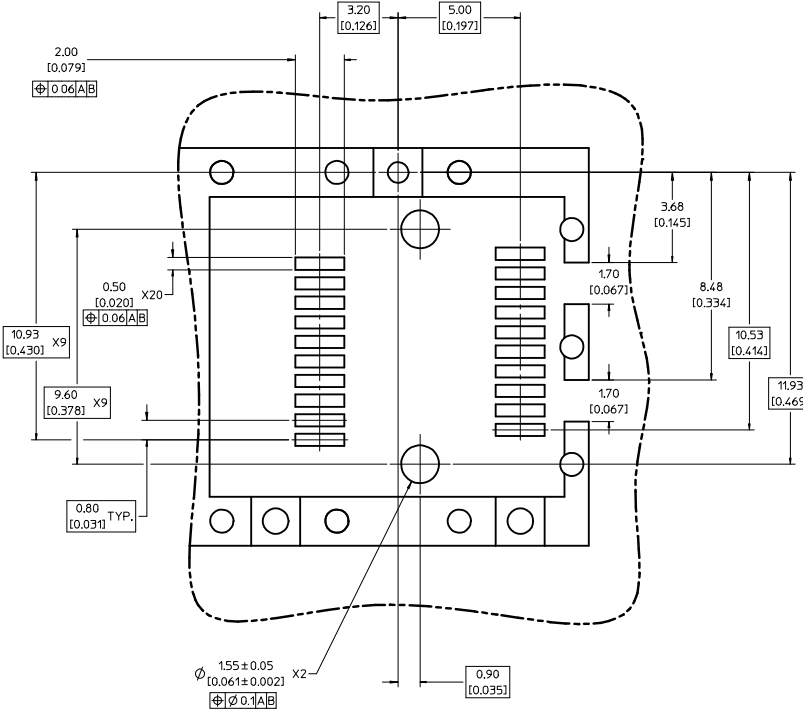
DETAIL1 SCALE 10:1
