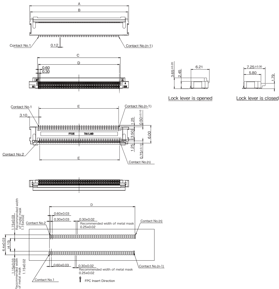
Recommended PCB Mounting Dimensions (Connector Mounting Side)
