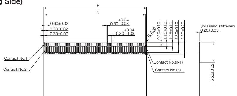
Recommended FPC Dimensions
