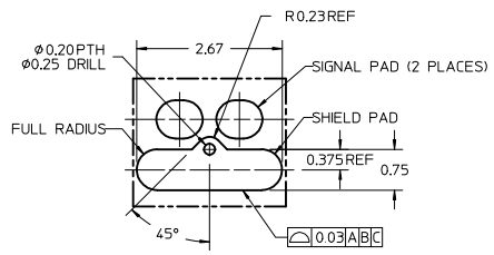
DETAIL 4 SCALE 20:1 (SOLDER MASK REMOVED TO REVEAL SHIELD TRACE)
