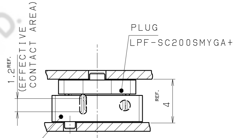
RECEPTACLE LPF-SC200SFYG (N) + MATED CONDITION (REF.) 嵌合状態図 (参考)
