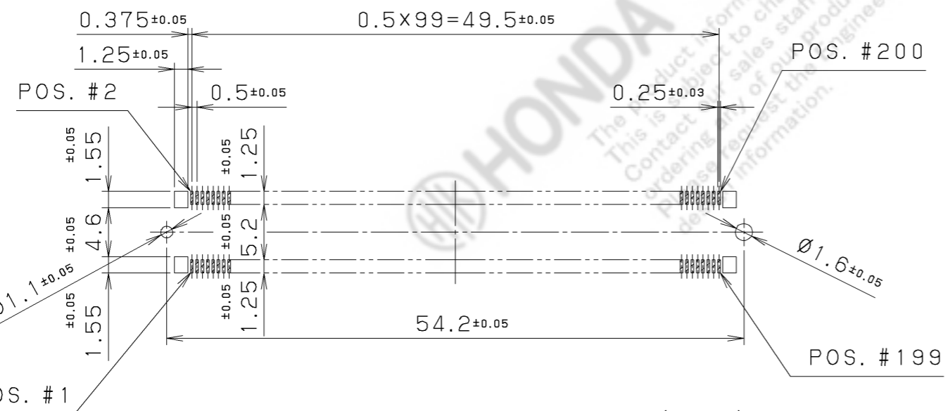
APPLICABLE P. C. BOARD DIMENSION (REF.) 適合基板寸法図 (参考)
