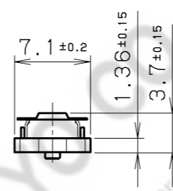
RECEPTACLE LPF-SC200SFYG (N) + MATED CONDITION (REF.) 嵌合状態図 (参考)
