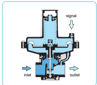
cross section RGB5
