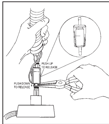
Figure 6. Air filter replacement.
