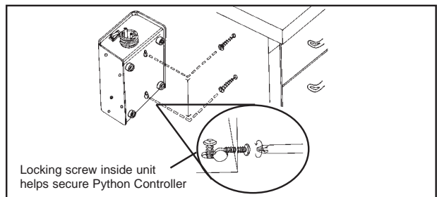
Figure 7. Installing controller to bench.
