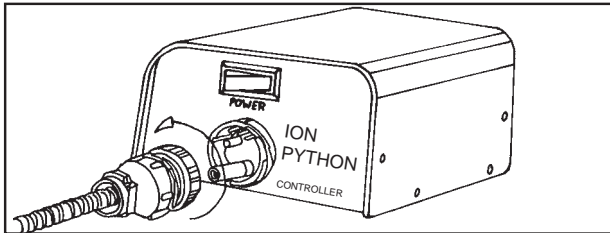
Figure 5. Replacing air nozzle assembly
