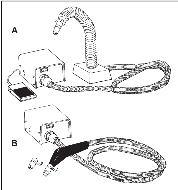
Figure 1. Desco EMIT Ion Python Air Nozzles A. Ion Python (Controller and Foot Switch) B. Hand Gun (Controller with Hose)
