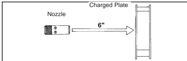
Figure 10. EOS/ESD S-3.1 decay time test set up.
