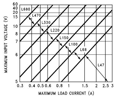
FIGURE 3. LM2576(HV)-3.3
