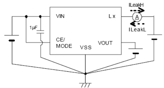
Circuit ⑥
