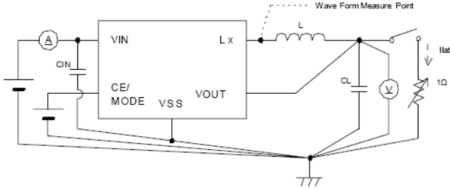
Circuit ⑨
