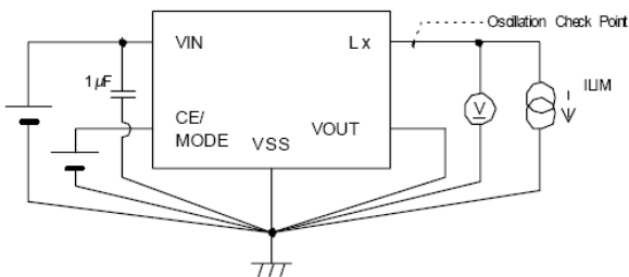
Circuit ⑦
