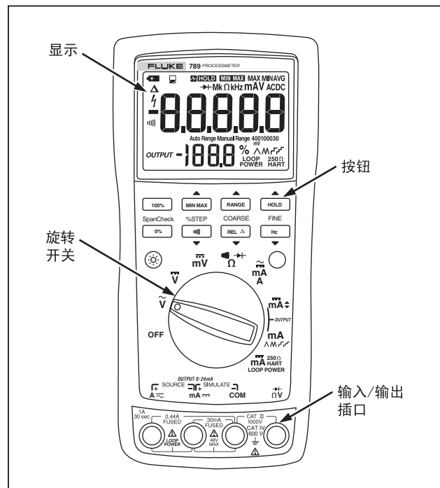
图 1. Fluke 789 ProcessMeter
