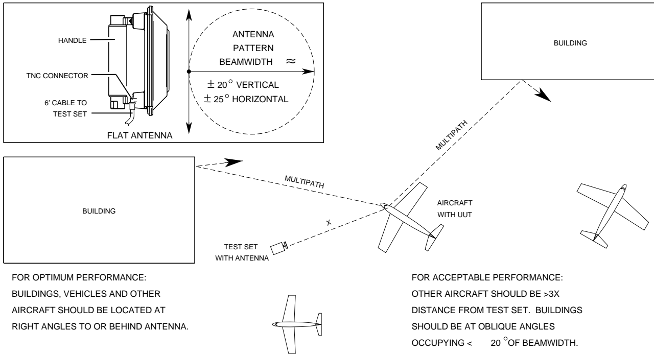
Suggested Layout to Reduce Multipath Errors Figure 11
