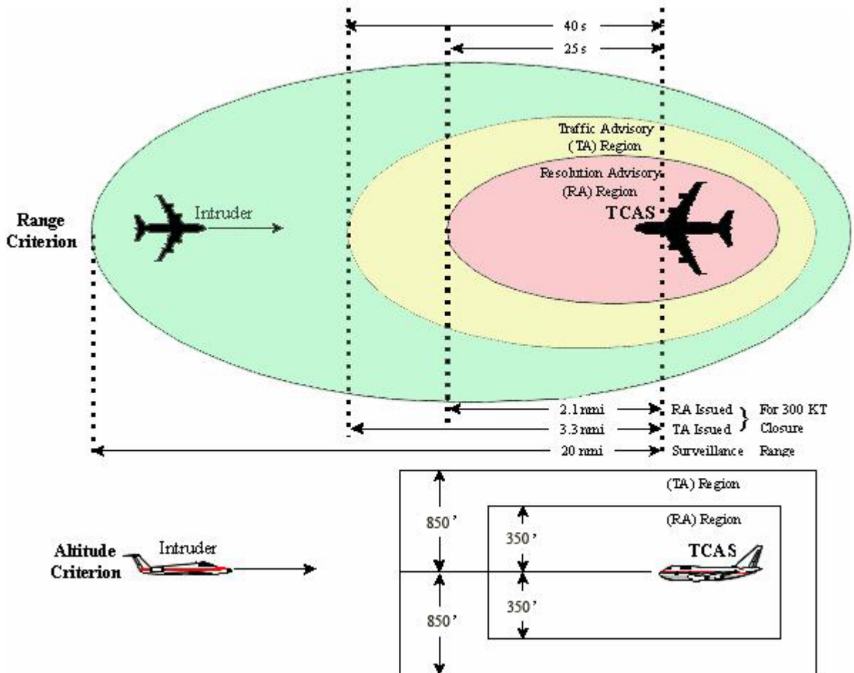
TCAS Protection Volume Example 5,000 ft to 10,000 ft Figure 7
