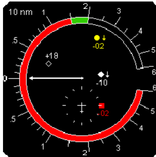
Typical TCAS II Display Figure 8
