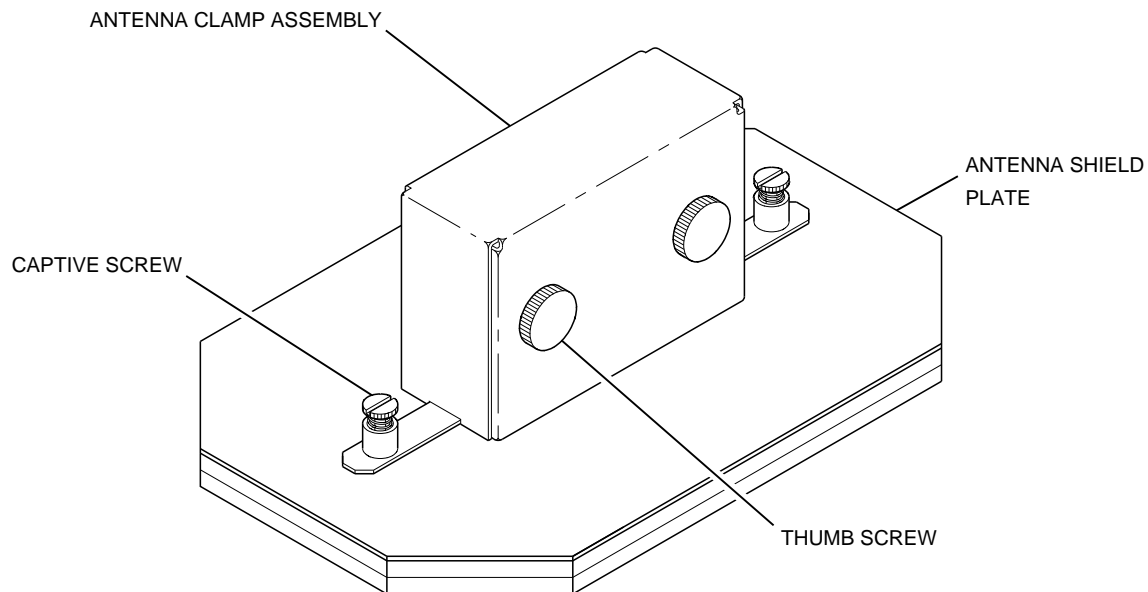
Antenna Shield Figure 2
