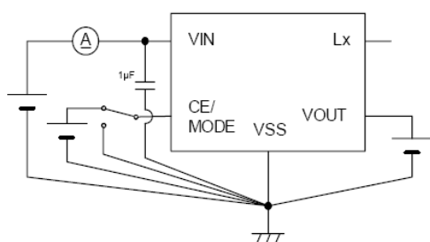
Circuit ⑤
