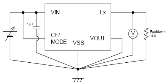
Circuit ④
