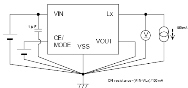
Circuit ⑤
