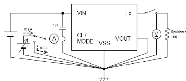
Circuit ⑧
