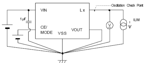
Circuit ⑦
