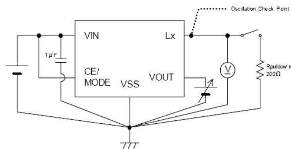
Circuit ④
