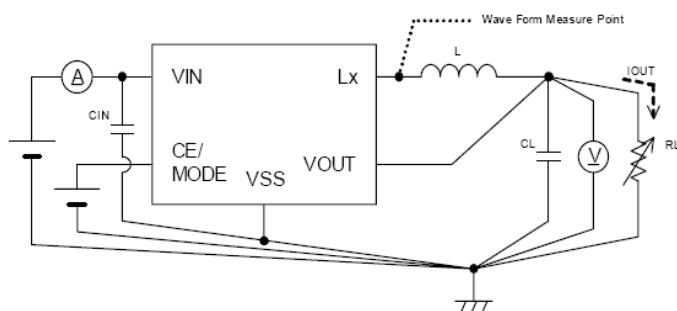
Circuit ①
