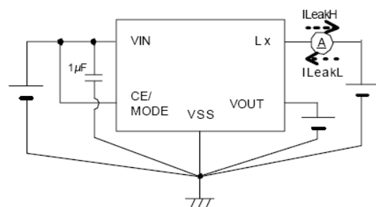
Circuit ⑥
