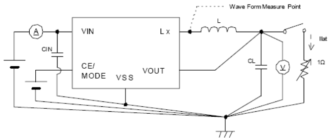
Circuit ⑨
