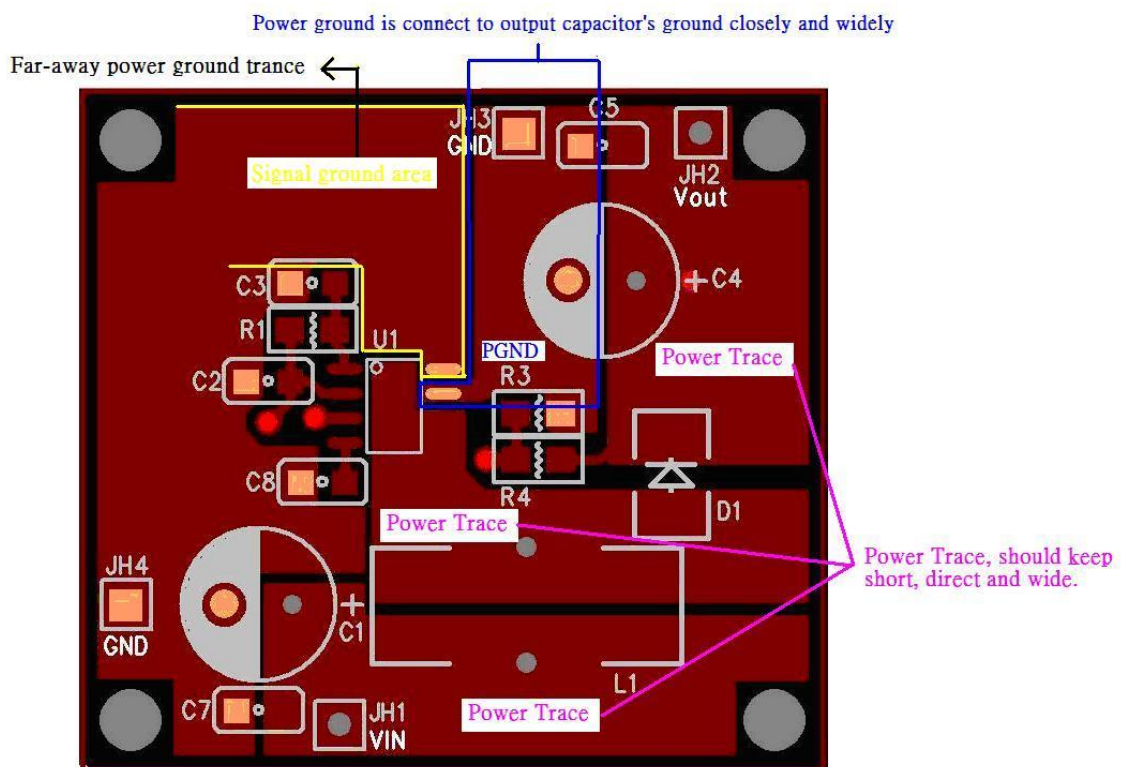
(AX5203 PCB Layout -Top View)
