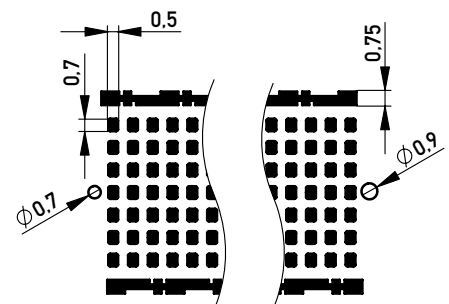
Recommended Layout
