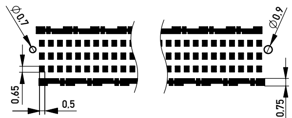
Recommended Layout
