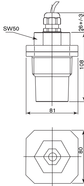
Remote ultrasonic probe 8170
