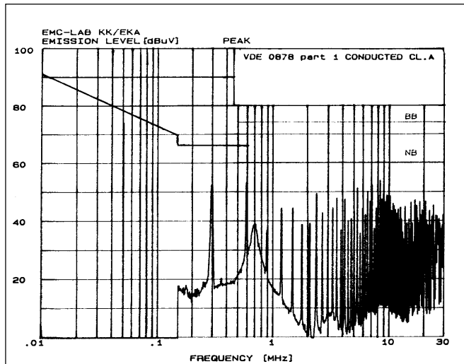
PKC series typical conducted EMI performance
